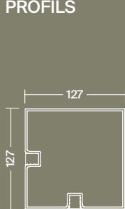
Post Pilier
