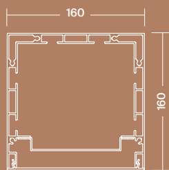
Post Pilier
