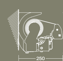
Wall installation 0° - 90° Installation murale 0° - 90°
