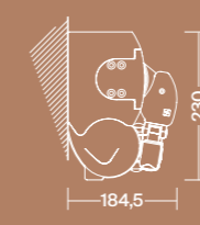
Wall installation 0° - 85° Installation murale 0° - 85°
