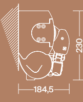
Wall installation 0° - 85° Installation murale 0° - 85°
