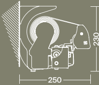
Wall installation 0° - 90° Installation murale 0° - 90°
