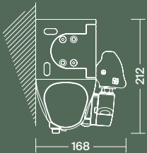
Wall installation 0° - 90° Installation murale 0° - 90°
