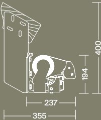
Installation between walls Installation entre murs
