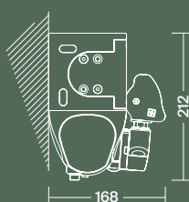
Wall installation 0° - 90° Installation murale 0° - 90°
