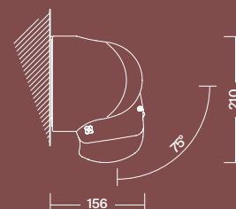
Wall installation 75° Installation murale 75°
